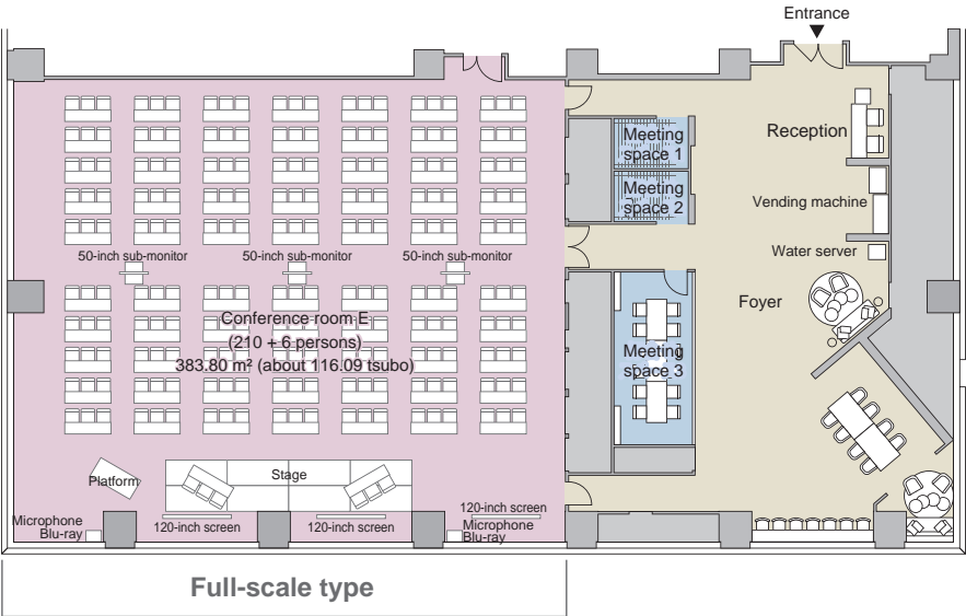
Standard classroom type plan
